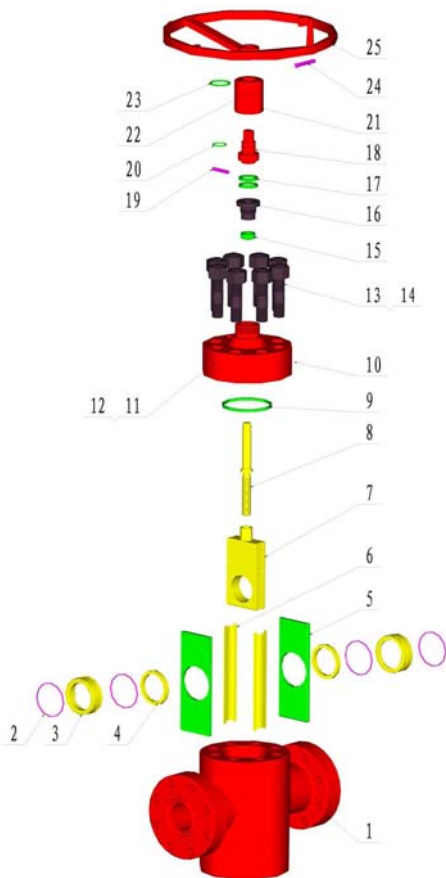
Manual Gate Valve
