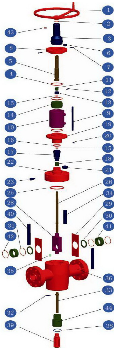
Hydraulic Gate Valve Break-Down List
